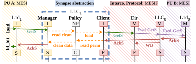
(a) Request to manager: propagating a load to the shared memory
