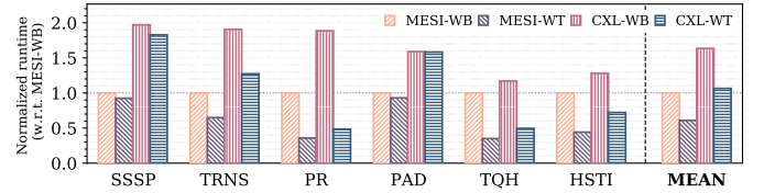
Fig. 11: Performance comparison between write-back and write-through policies for MESI and CXL off-core protocols in the hetero-chiplets scenario.
