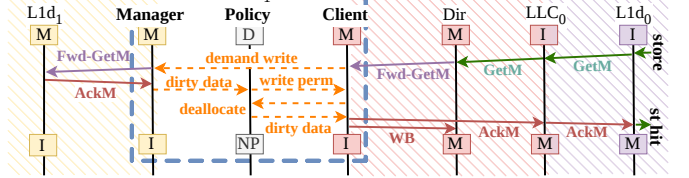
(b) Request to client: forwarding a store from the shared memory.
