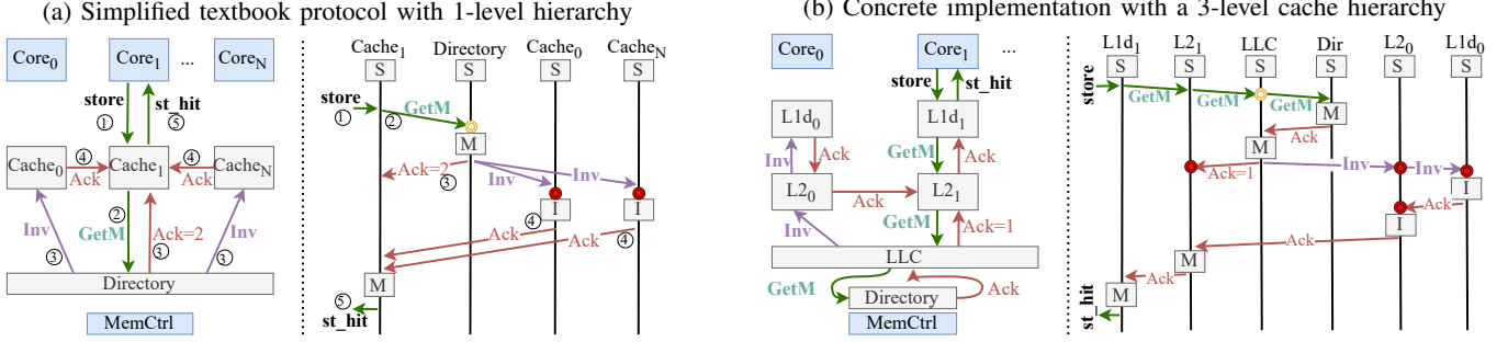
Fig. 1: Coherence transaction flow for store operation from Core 1 . Left parts shows system architecture. Right parts the matching protocol message flows and controller state transitions. Red dots mark race points and the yellow point the serialization point.
