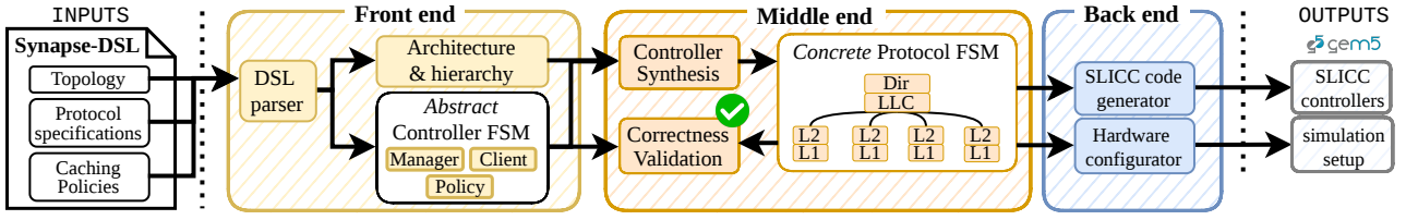
Fig. 5: The SYNAPSE pipeline. It takes as input coherence protocol, caching policy, and topology specifications, to generate all SLICC controllers in the hierarchy, enabling performance evaluation of CCPs in gem5 simulations.
