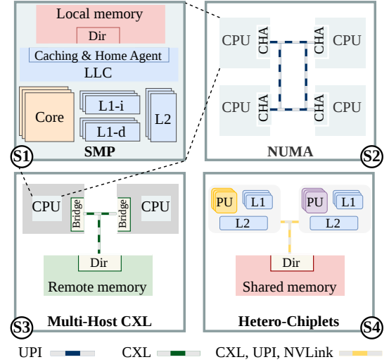
Fig. 2: Four typical cache coherence scenarios in modern architectures.
