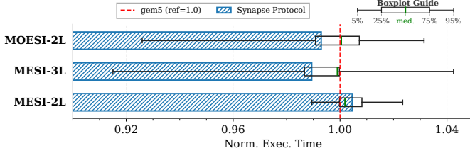
Fig. 8: Mean normalized execution time of Synapse-synthesized vs. gem5 manual (library) implementations across 30 workloads.
