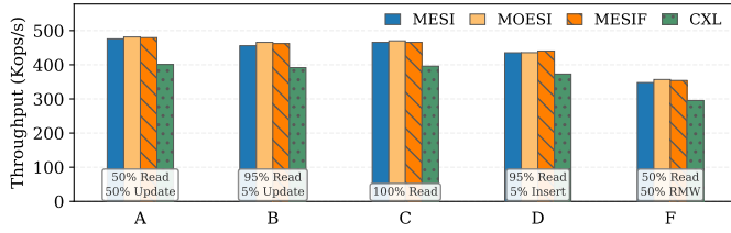
Fig. 10: Throughput (Kops/s) of four inter-node bridge protocol configurations in the multi-host CXL scenario across five YCSB workloads.
